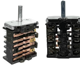
F/006 6 Position EGO Stove Switch
