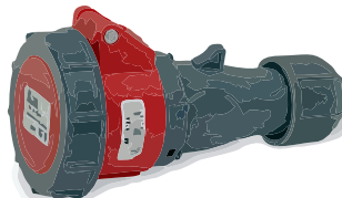
CEE COUPLER 16A 5P 380V Ip44
